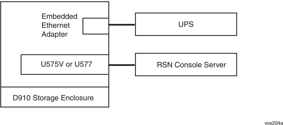
Figure 3-3. ftServer V 100, V 200, and V 400 Module Base Configuration
