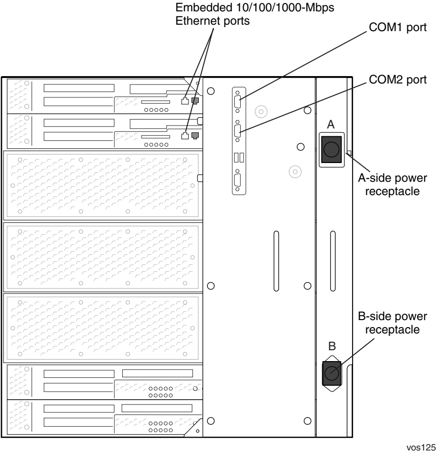
Figure A-2. ftServer V 200 and V 400 Systems Backplane: Rear View
