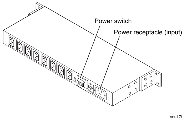
Figure A-6. AAP41104V PDU
