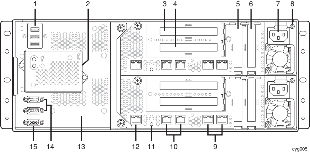
Figure A-2. ftServer 27x0, 47x0, 64x0 System: Rear View
