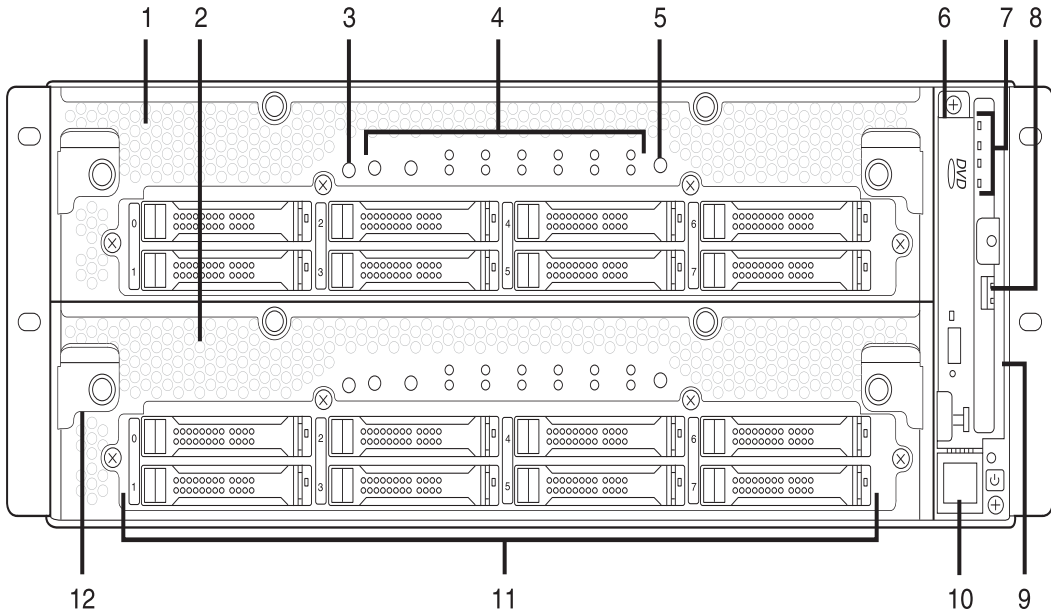
Figure A-1. ftServer 27x0, 47x0, 64x0 System: CPU-I/O Enclosures: Front View
