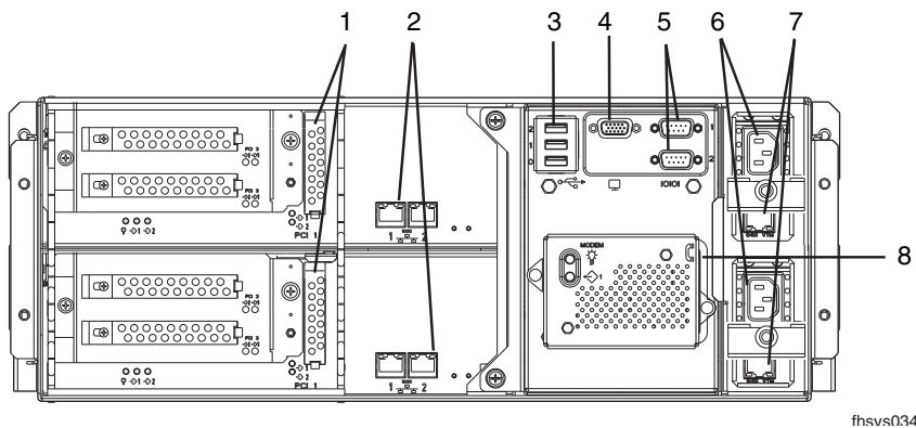
Figure A-5. Rack-Mountable ftServer 2510, 4410, or 6210 System (With VTMs): Rear View
