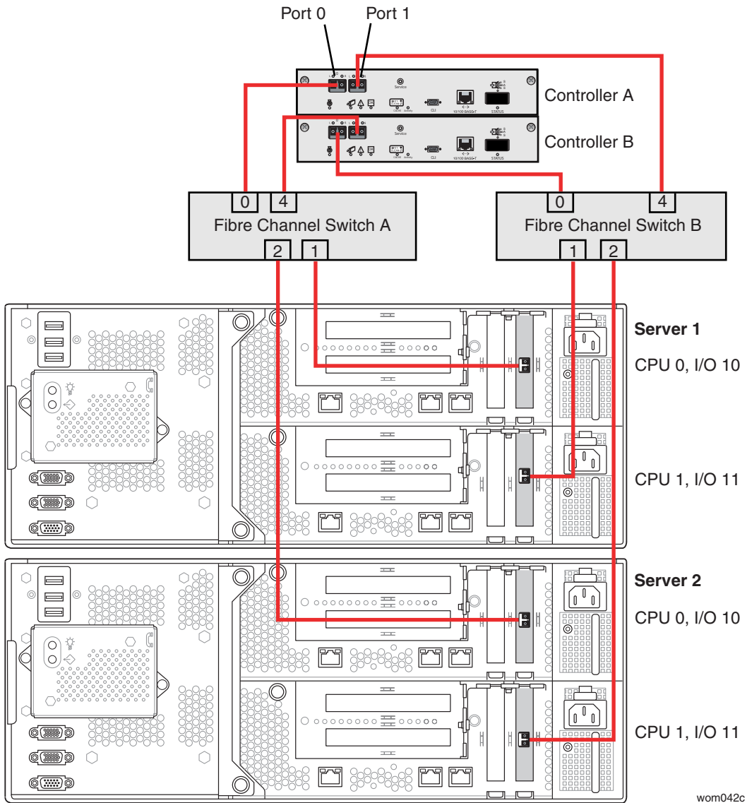
Figure 4-3. Fibre Channel Connections to an ftScalable Storage G2 or First-Generation ftScalable Storage System in a SAN Configuration
