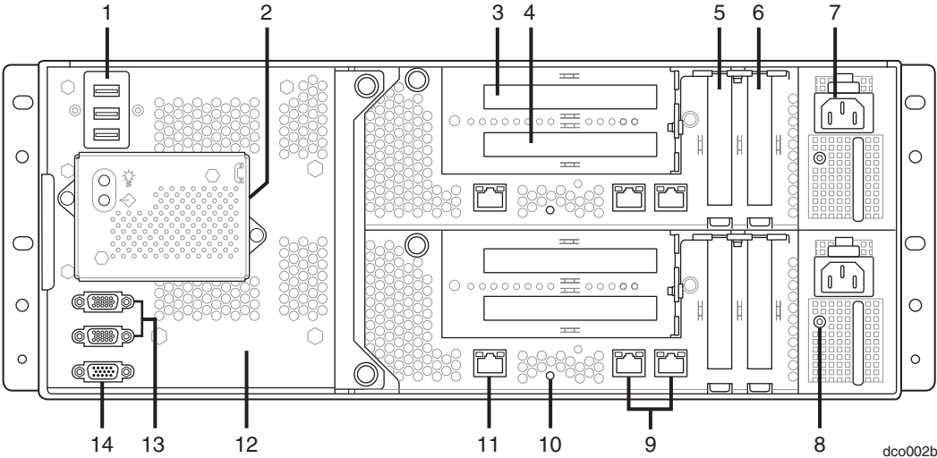
Figure A-2. ftServer 2600, 4500, 6300, or 6310 System: Rear View
