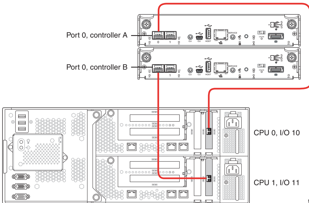
Figure 4-1. Fibre Channel Connections to an ftScalable Storage G2 System in a DAS Configuration
