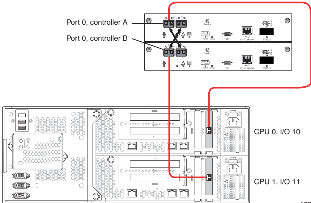
Figure 4-2. Fibre Channel Connections to a First-Generation ftScalable Storage System in a DAS Configuration*
