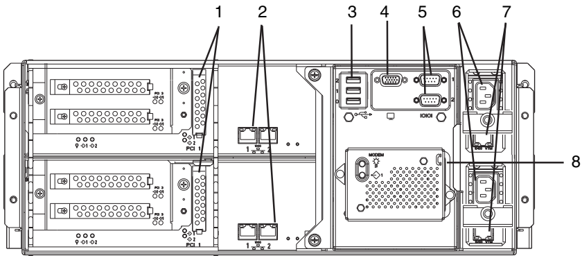
Figure A-5. Rack-Mountable ftServer 2510, 4410, or 6210 System (With VTMs): Rear View
