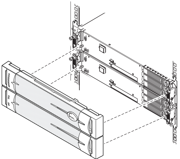
Figure A-4. Rack-Mountable ftServer 2510, 4410, or 6210 System: Front View
