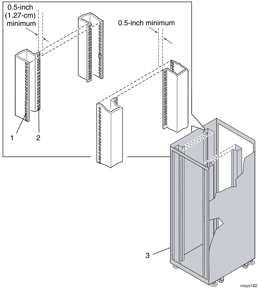
Figure 6-1. Rail Clearance
